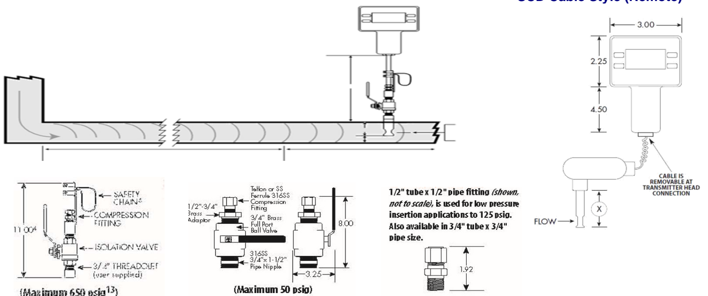
SCD Cable Style (Remote)
